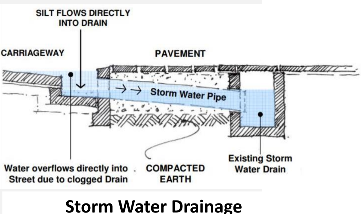
Storm Water Drainage
