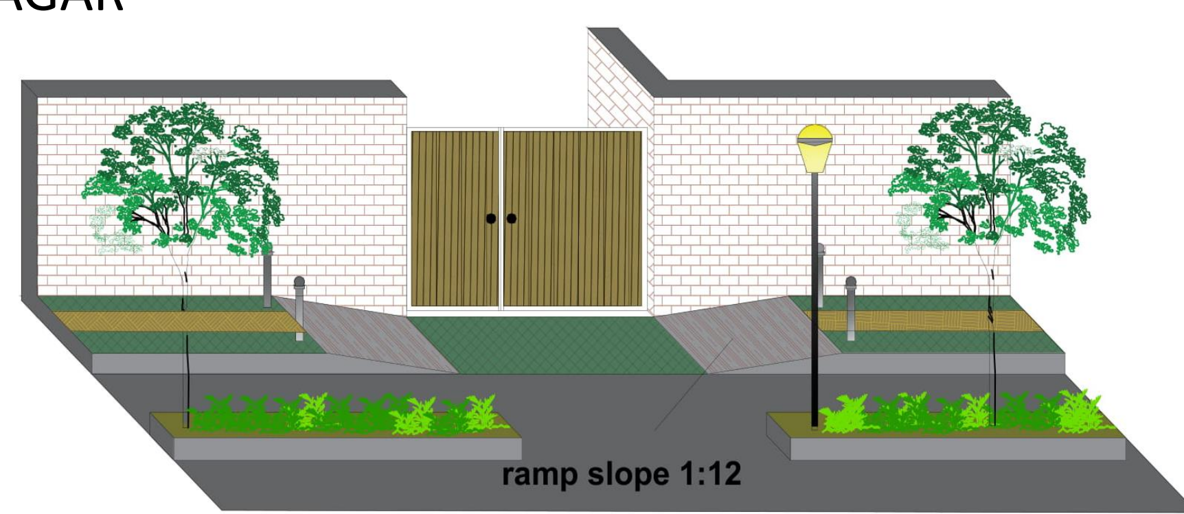
Ramps in front of Residence gates ramp slope 1:12
